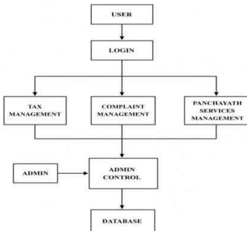
Figure 4.1: System working
