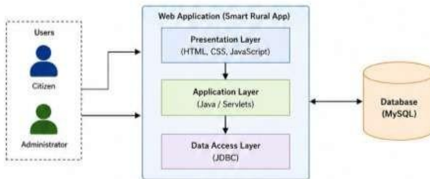
Figure 4.2: System Architecture
